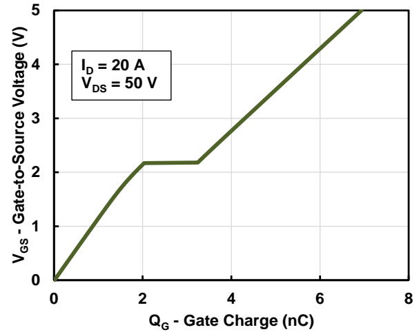
Figure 6b: EPC2104-Q2: Gate Charge
