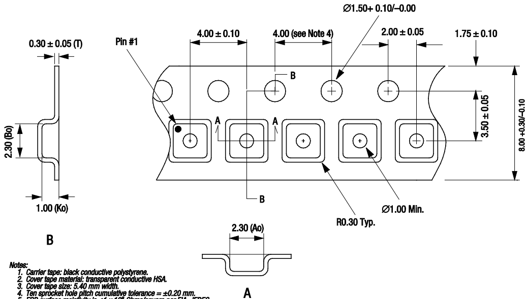
Figure 18. SKY65094-360LF Tape and Reel Dimensions
