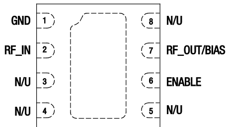
Figure 2. SKY65094-360LF Pinout – 8-Pin DFN Package (Top View)
