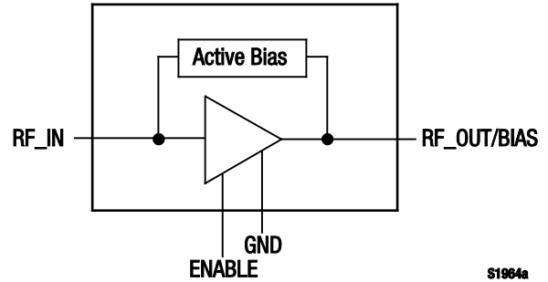
Figure 1. SKY65094-360LF Functional Block Diagram
