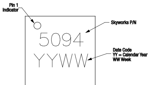
Figure 16. Typical Case Markings (Top View)
